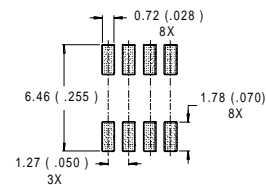
RECOMMENDED FOOTPRINT
