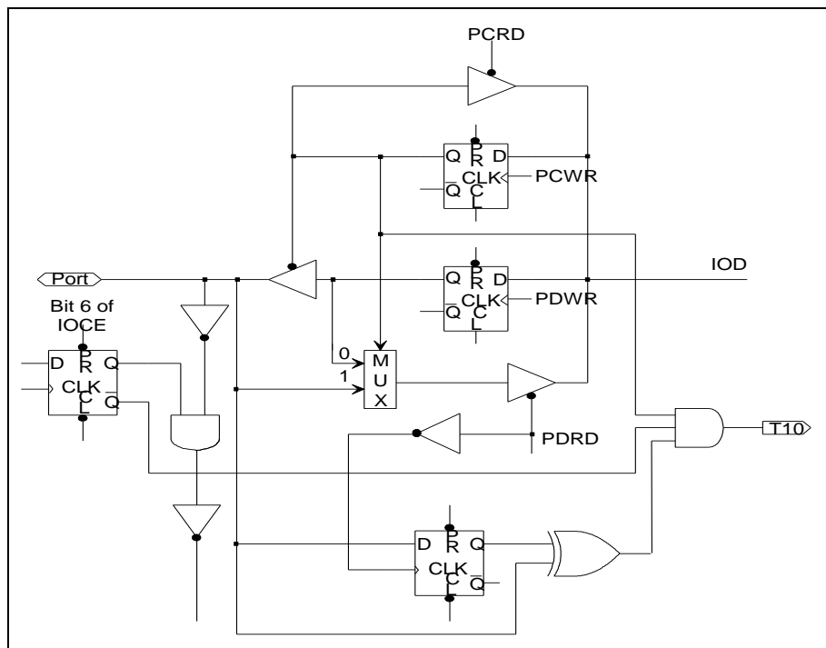
Figure 5-5 I/O Port and I/O Control Register Circuit for Port 5
