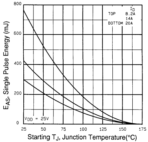
Fig 13c. Maximum Avalanche Energy Vs. Drain Current
