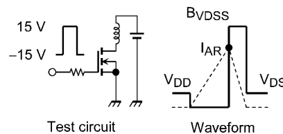
Fig. 8.16 Test Circuit/Waveform
