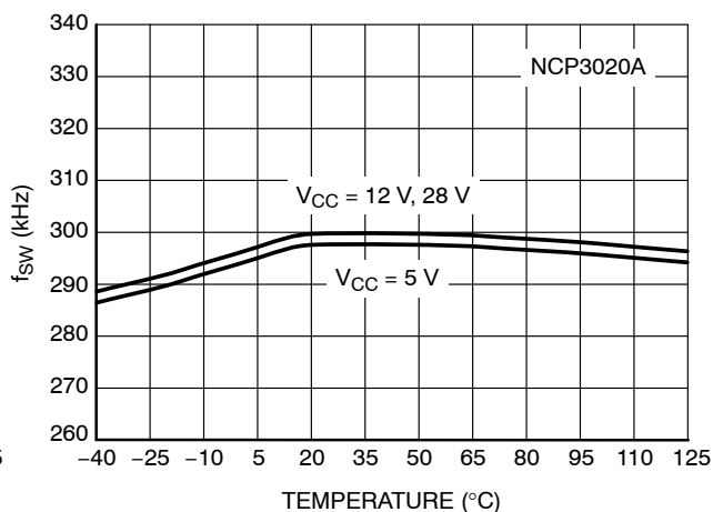
Figure 8. Switching Frequency vs. Input Voltage and Temperature
