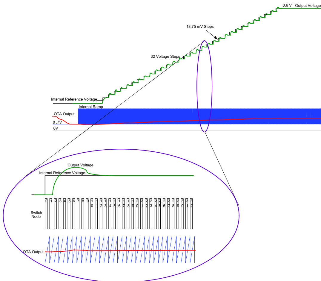
Figure 21. Soft-Start Details
