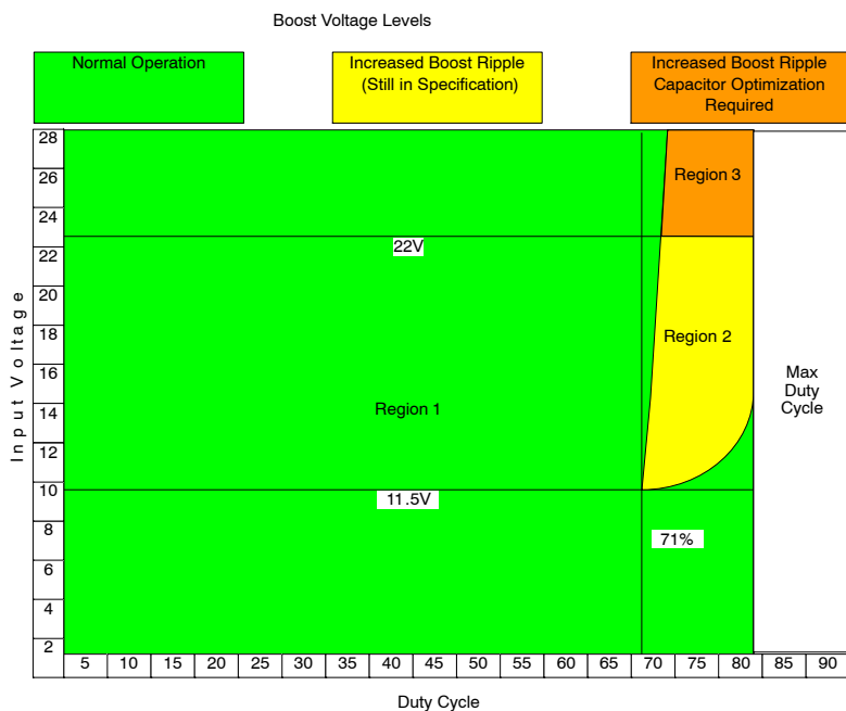
Figure 29. Safe Operating Area for Boost Voltage with a 0.1 \mu\text{F} Capacitor
