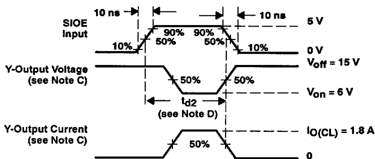
VOLTAGE WAVEFORMS
