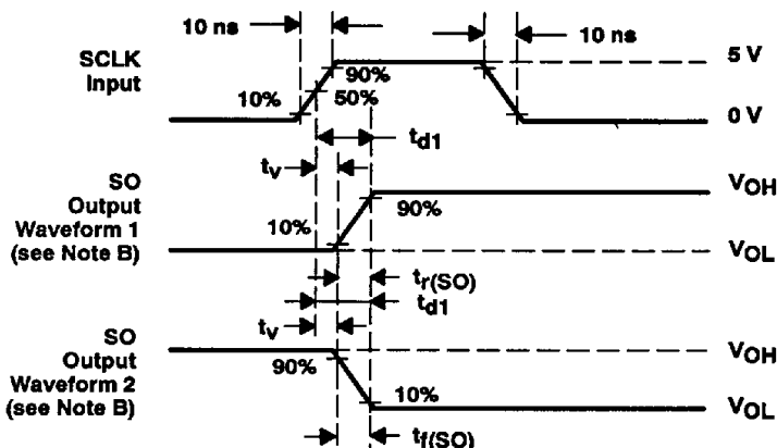
VOLTAGE WAVEFORMS
