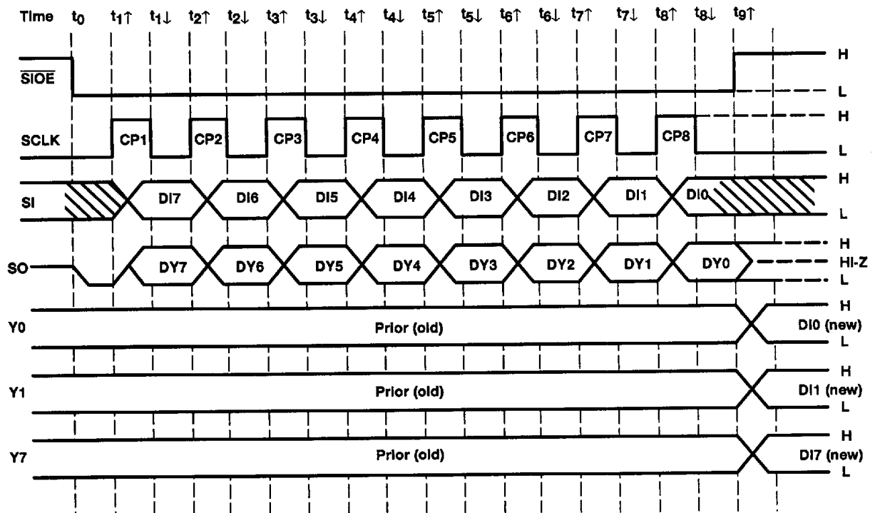
Figure 10. Data-Byte Transfer Timing
