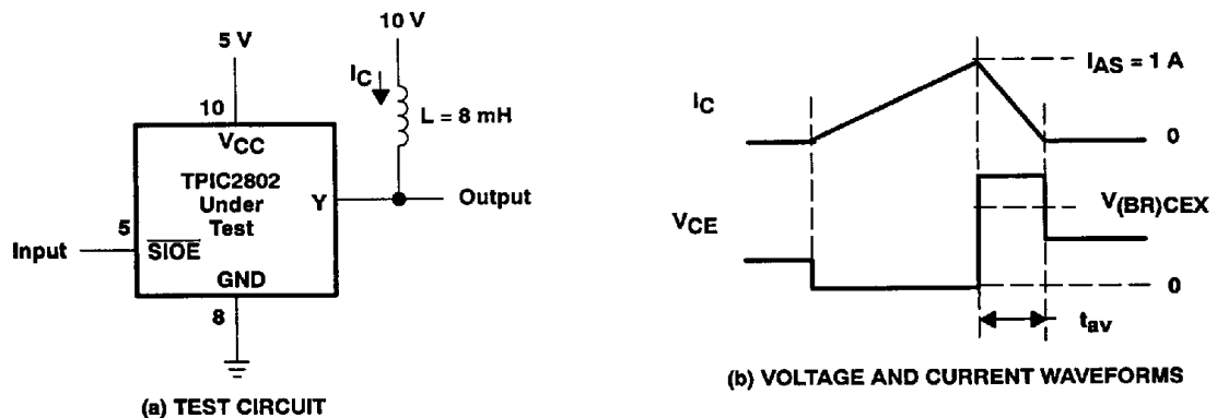
Figure 6. Single-Pulse Avalanche Energy Test Circuit and Waveforms
