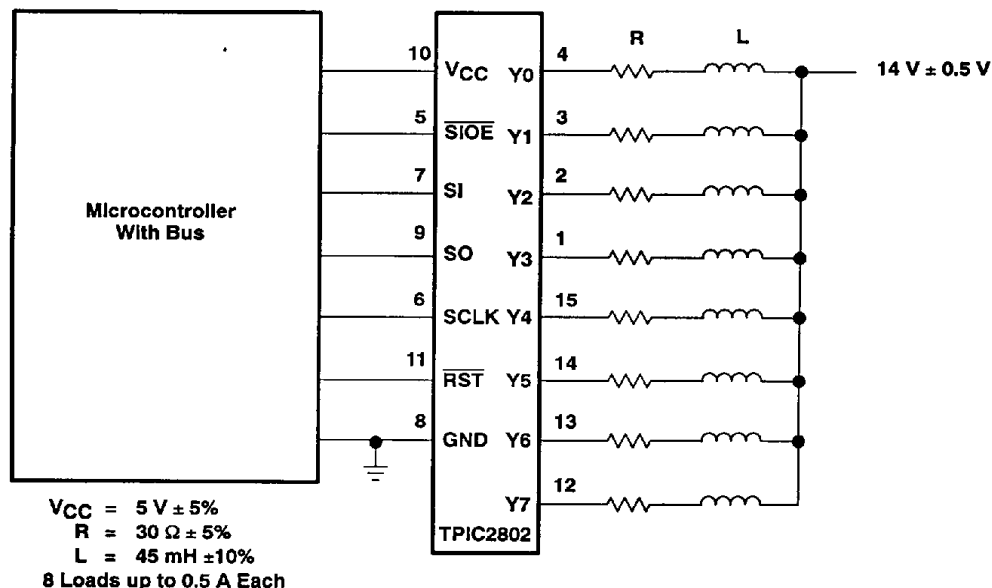
Figure 9. Microcontroller Driving Eight Loads Using a TPIC2802 for Load Interface
