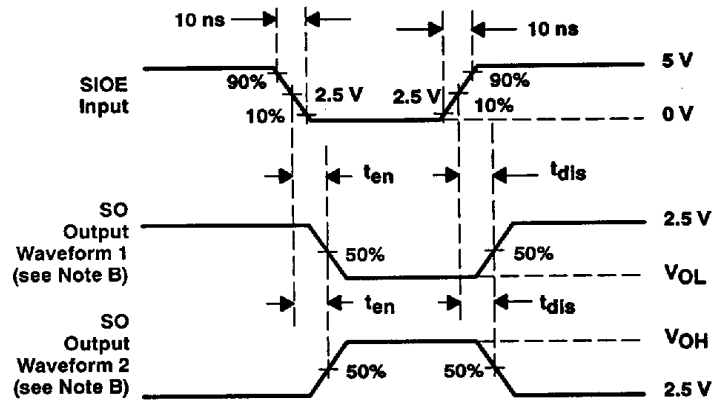
VOLTAGE WAVEFORMS
