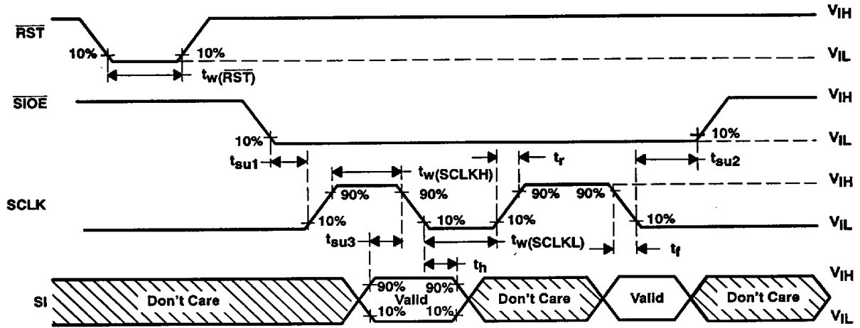
Figure 1. Input Timing Waveforms
