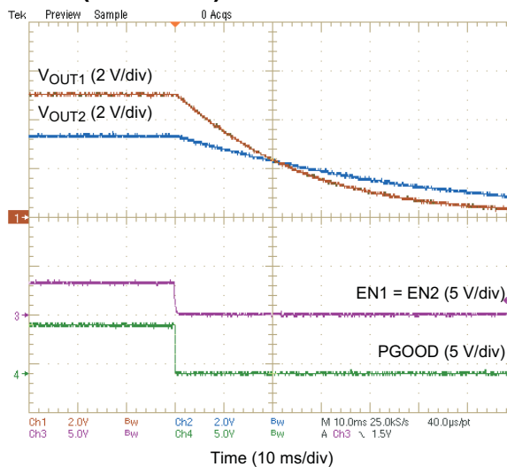
Figure 24. Output Discharge
