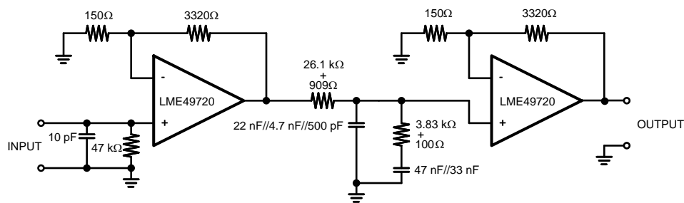
Figure 1. Passively Equalized RIAA Phono Preamp
