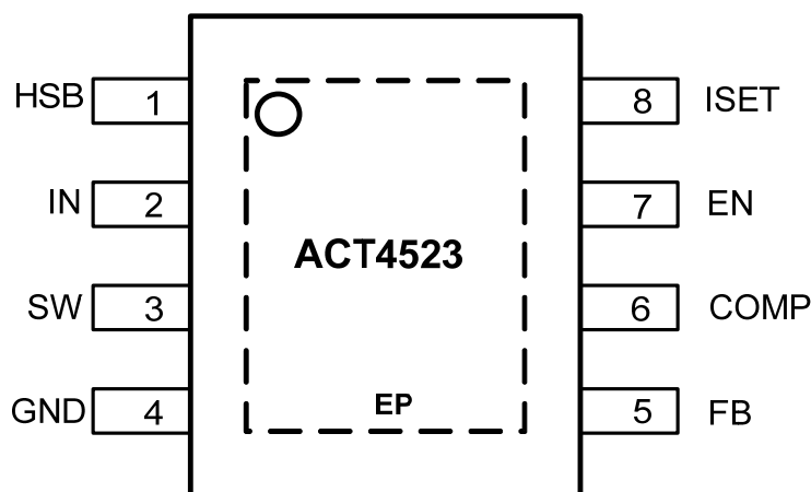
SOP-8EP
