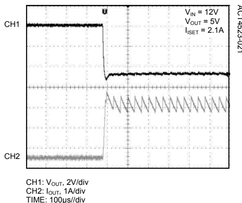
Short Circuit
