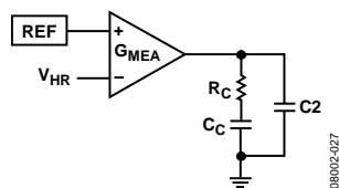
Figure 27. Compensation Components
