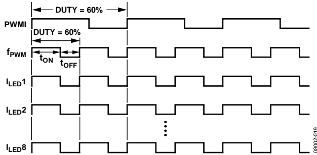
Figure 19. No Delay PWM Dimming Timing
