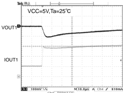
Fig.20 VOUT1 transient response ( I_o 0.5A \rightarrow 1.5A / usec)
