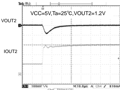
Fig.22 VOUT2 transient response ( I_o 0.5A \rightarrow 1.5A / usec)
