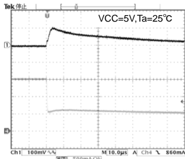
Fig.21 VOUT1 transient response ( I_o 1.5A \rightarrow 0.5A / usec)
