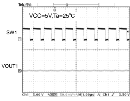
Fig.17 SW1 wave form ( I_o=1.5A )
