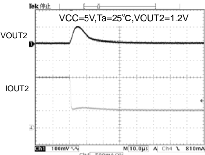
Fig.23 VOUT2 transient response ( I_o 1.5A \rightarrow 0.5A / usec)
