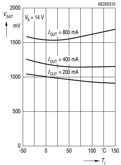
Total Drop at outputs V_{SAT} over Temperature
