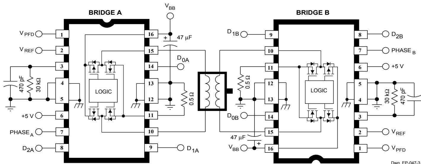
Figure 4 — Typical Application
