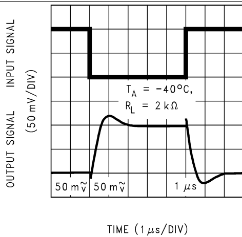
Figure 43. Inverting Small Signal Pulse Response
