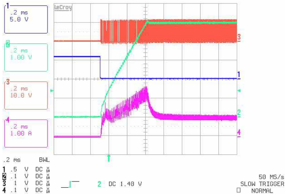
Fig1. 5V/2A Output
