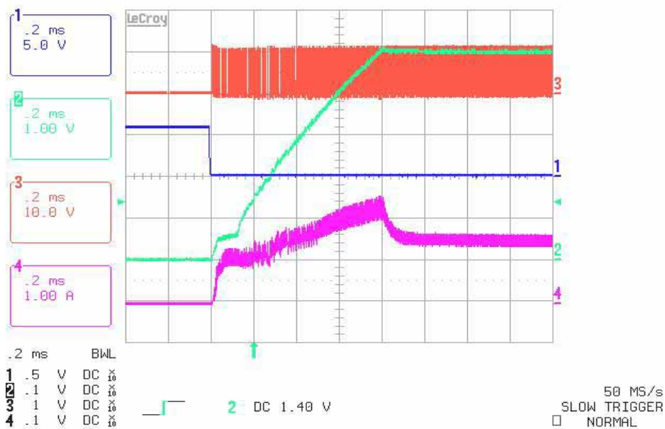
Fig2. 5V/3A Output
