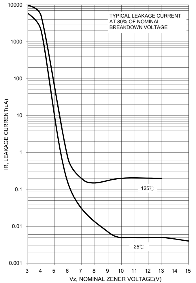
FIG.5 TYPICAL LEAKAGE CURRENT
