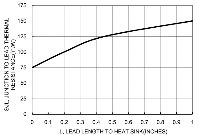
FIG. 10 TYPICAL THERMAL RESISTANCE versus LEAD LENGTH
