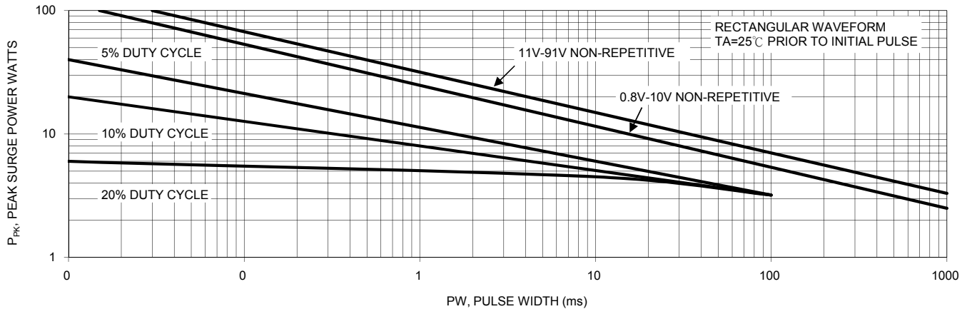
FIG.11 MAXIMUM SURGE POWER
