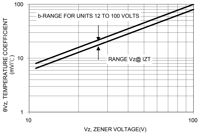
FIG.8 TEMPERATURE COEFFICIENTS
