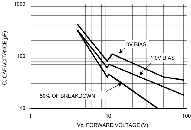
FIG.6 TYPICAL CAPACITANCE versus Vz
