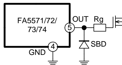
Fig.32 Minus voltage protection circuit
