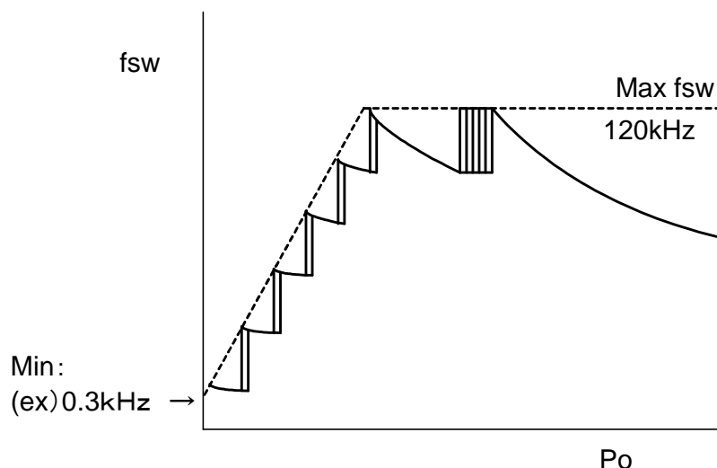
Fig. 5 Oscillation frequency ( f_{sw} ) vs output power characteristics ( P_o )
