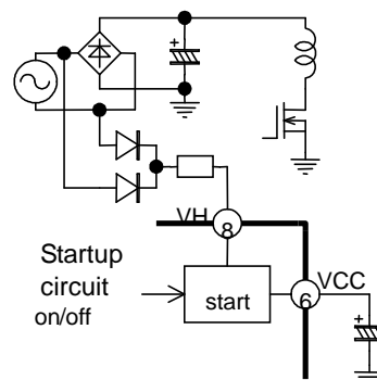
Fig.26 VH pin circuit (3)
