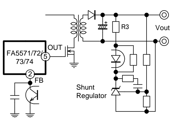
Fig. 40 Changing the burst frequency
