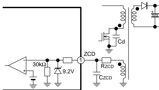
Fig.11 ZCD pin circuit
