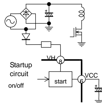
Fig.25 VH pin circuit (2)
