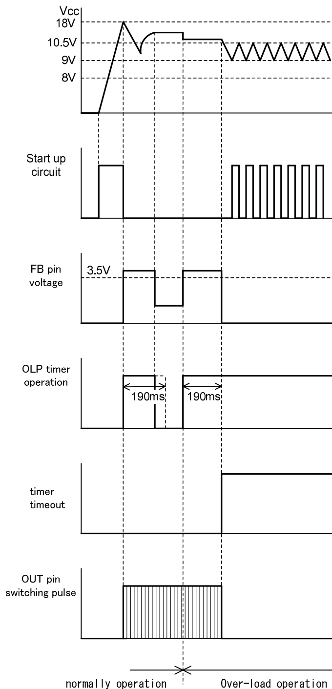
Fig.10 Operation at overload (FA5572/74)
