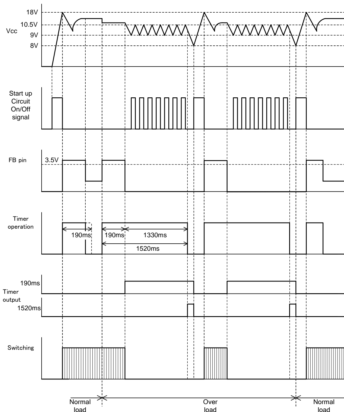
Fig.9 Operation at overload (FA5571/71A/73/70/5671)
