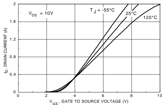
Figure 5. Transfer Characteristics.
