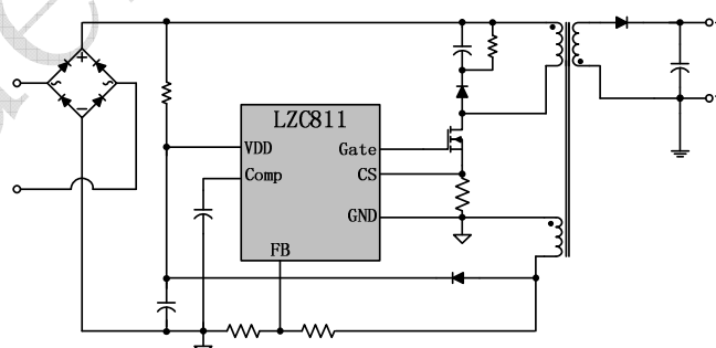
Fig 1 Application Circuit
