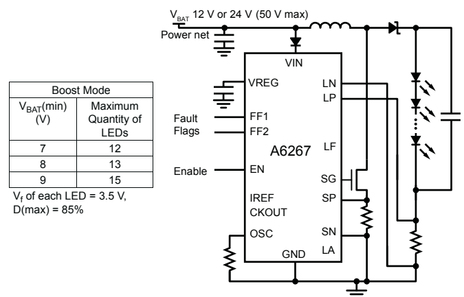
Boost Mode
