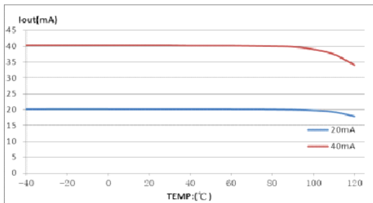
Diagram 5. SM2082B Output Current Temperature Characteristics ( I_{OUT} = 20\text{mA} 和 40\text{mA} )
