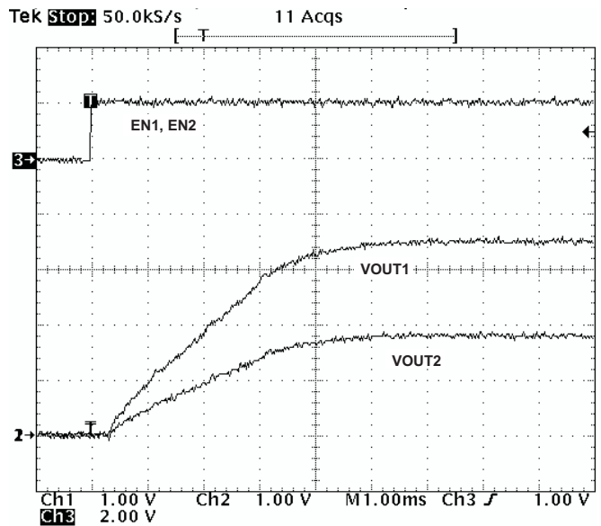
Figure 34. Ratiometric Start-Up using Coupled SS/TR Pins
