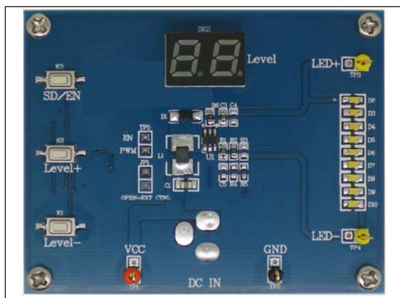
Figure 1: Photo of IS31BL3508A Evaluation Board
