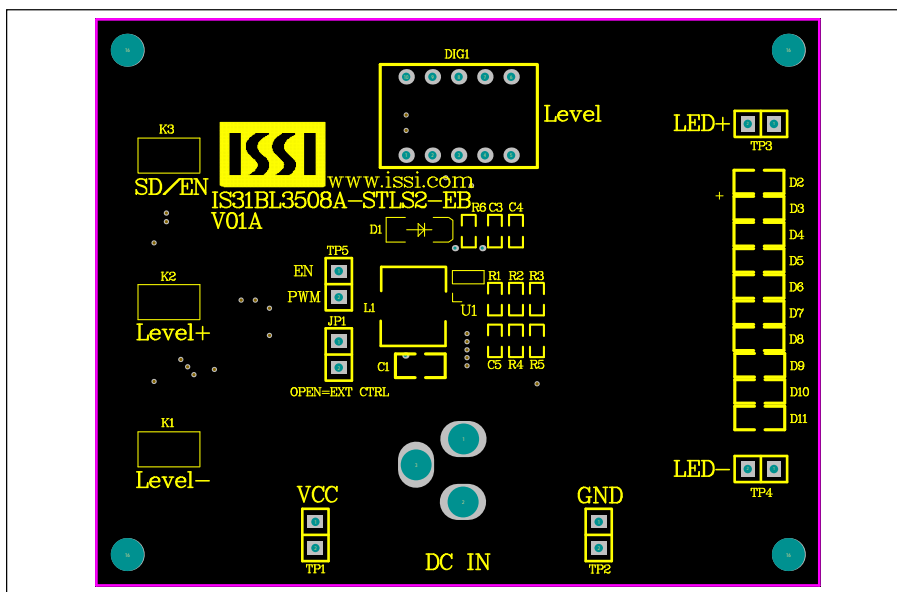
Figure 3: Board Component Placement Guide - Top Layer
