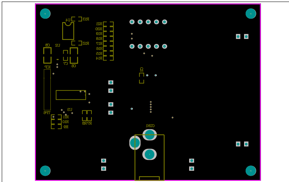
Figure 5: Board Component Placement Guide -Bottom Layer
