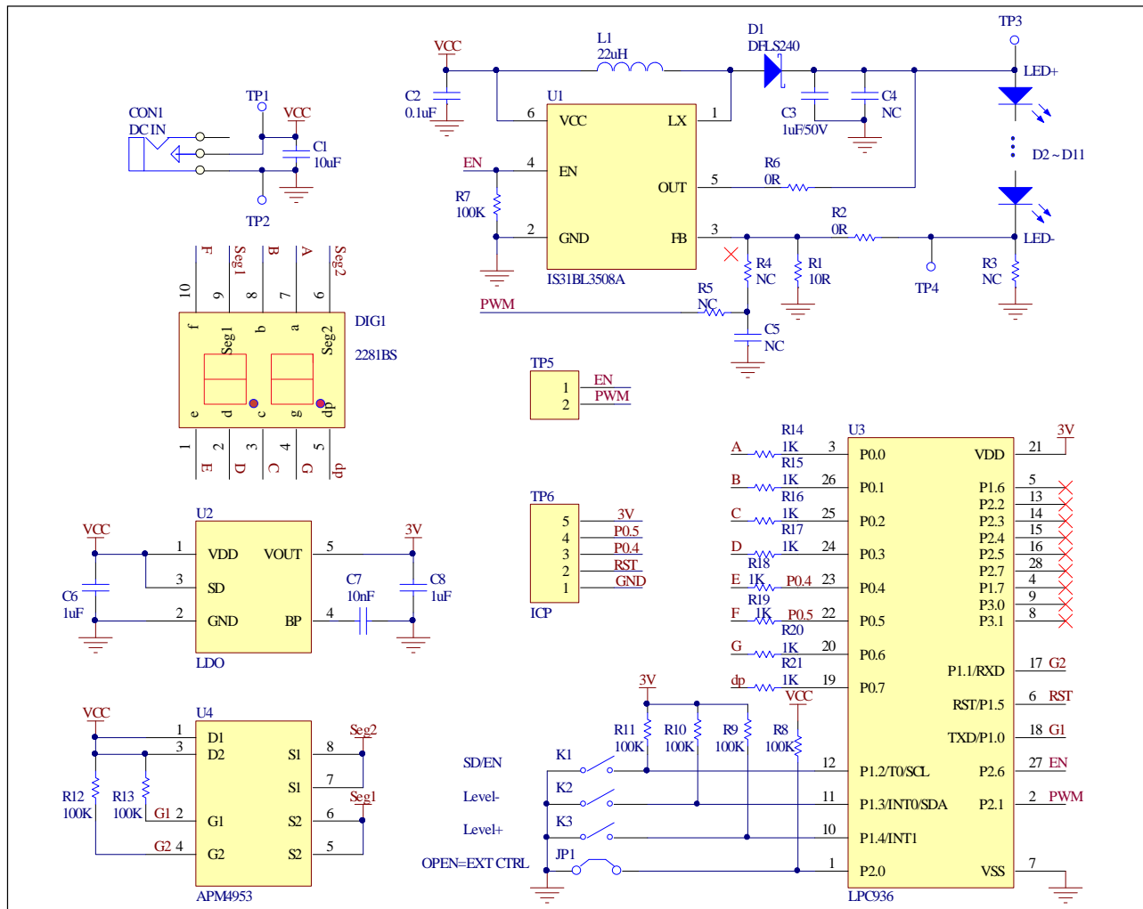
Figure 2: IS31BL3508A Application Schematic
