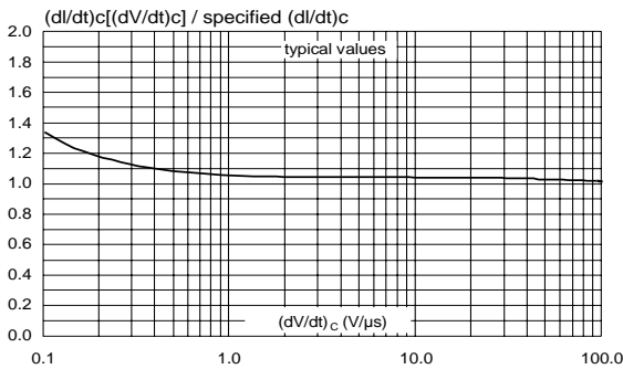
Figure 9: Relative variation of critical rate of decrease of main current (dI/dt)_c versus reapplied (dV/dt)_c
