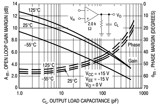
Figure 27. Open Loop Gain Margin and Phase Margin versus Output Load Capacitance
