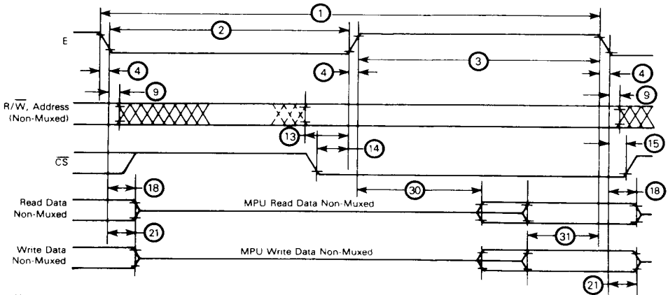
FIGURE 1 — BUS TIMING
