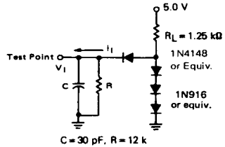
FIGURE 5 -- NMOS EQUIVALENT TEST LOAD
