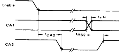
FIGURE 8 -- CA2 DELAY TIME (Read Mode; CRA-5=1, CRA-3=CRA-4=0)
