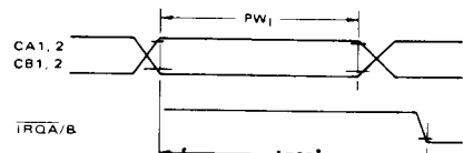
FIGURE 13 -- INTERRUPT PULSE WIDTH AND \overline{IRQ} RESPONSE
