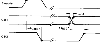
FIGURE 12 -- CB2 DELAY TIME (Write Mode; CRB-5=1, CRB-3=CRB-4=0)
