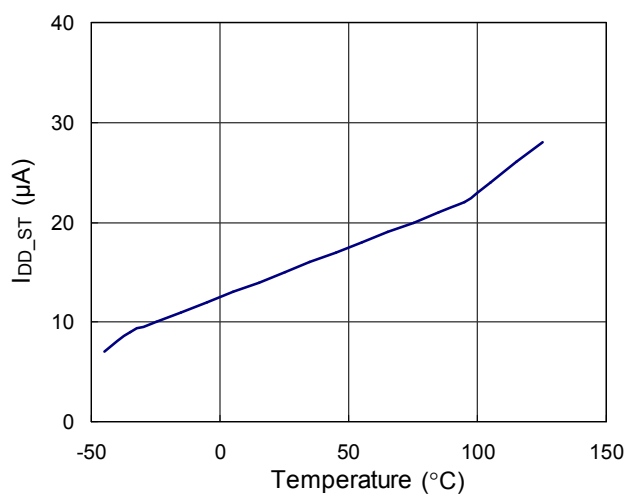
Startup Current vs. Temperature
