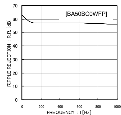
Fig.6 Ripple Rejection
