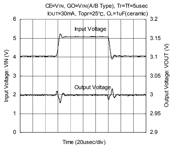
XC6217x302
