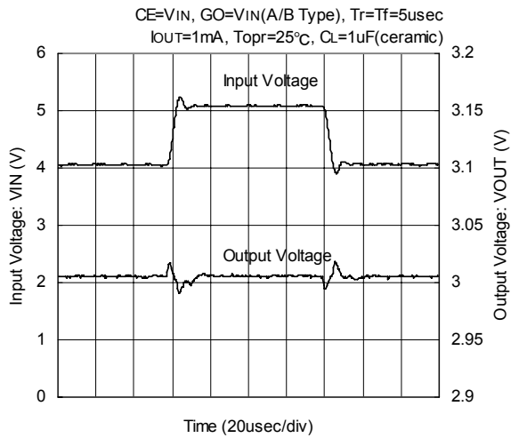
XC6217x302
