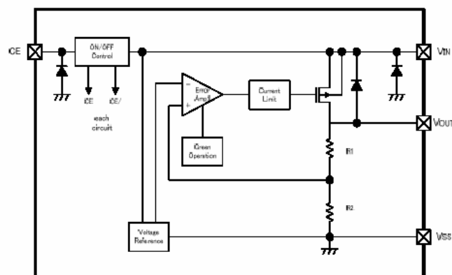
● XC6217C Series
