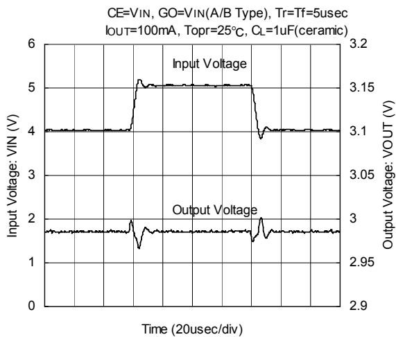
XC6217x302
