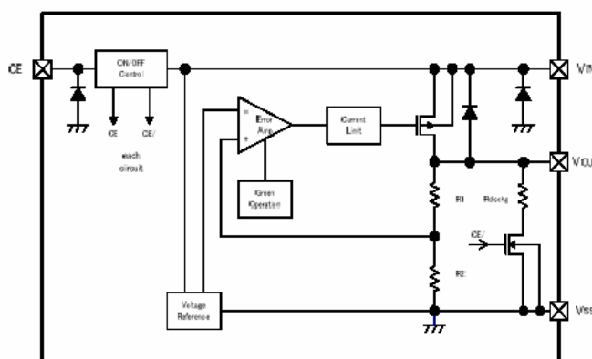
● XC6217D Series
