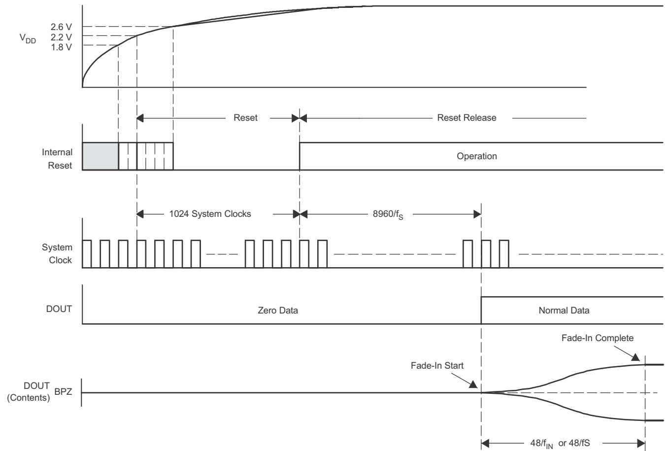
Figure 2. Power-On Timing
