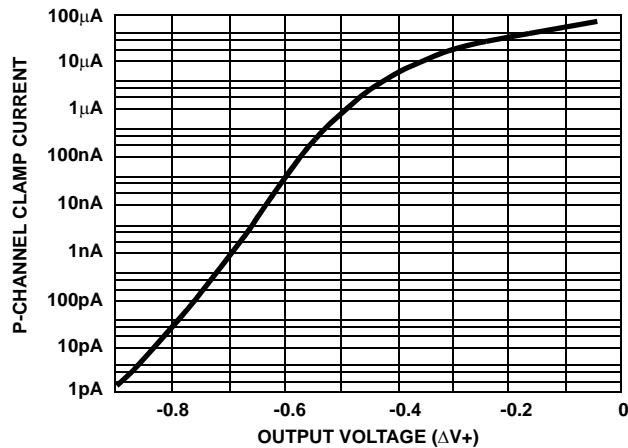
FIGURE 21. P-CHANNEL CLAMP CURRENT vs OUTPUT VOLTAGE
