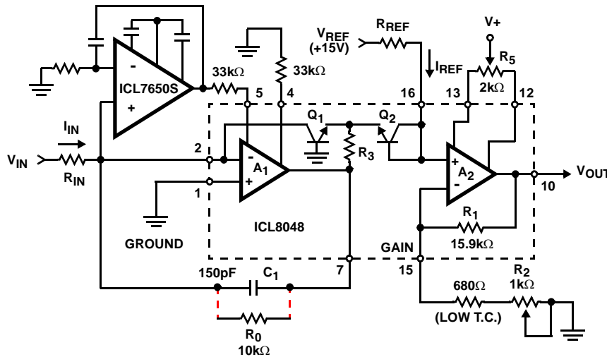
FIGURE 6. ICL8048 OFFSET NULLED BY ICL7650S
