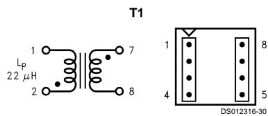
FIGURE 15. Coilcraft Q4434-B
