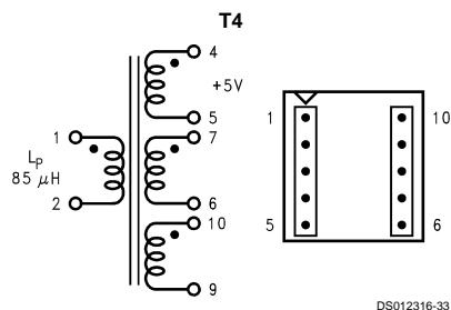
FIGURE 18. Coilcraft Q4344-B
