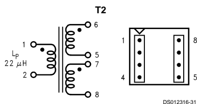
FIGURE 16. Coilcraft Q4337-B
