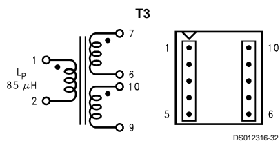
FIGURE 17. Coilcraft Q4343-B
