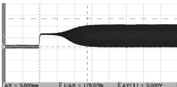
32768Hz Crystal
