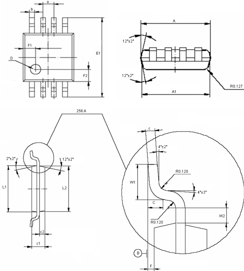
Figure 8 VA7208 8-Pin MSOP Package
