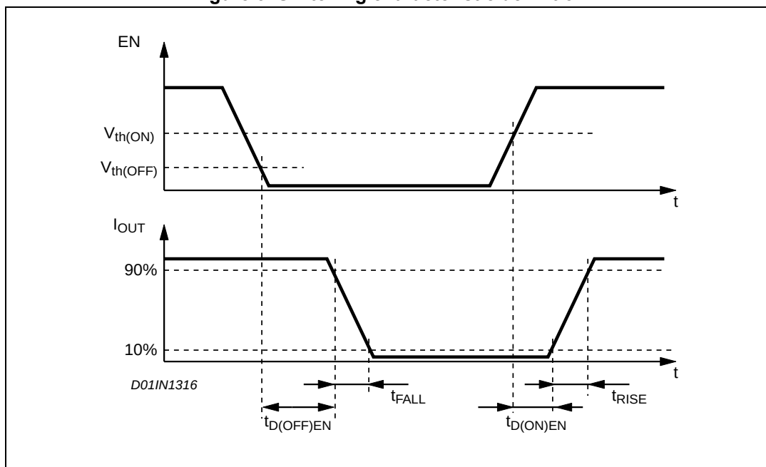
Figure 3. Switching characteristic definition
