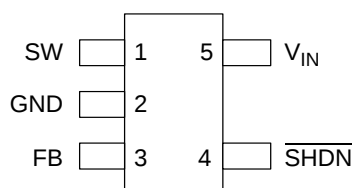
Figure 2. Pin Configuration of AP3012 (Top View)
