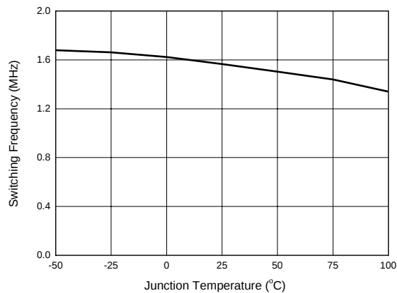
Figure 6. Switching Frequency vs. Junction Temperature
