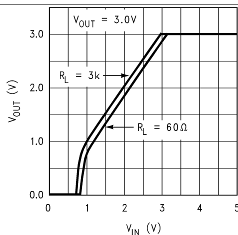
Figure 6. Dropout Characteristics
