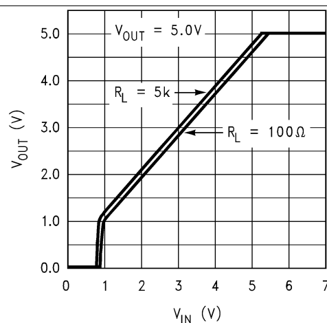
Figure 4. Dropout Characteristics
