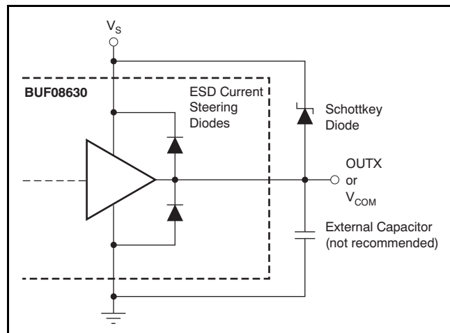
Figure 36. Output Pins ESD Protection Current-Steering Diodes
