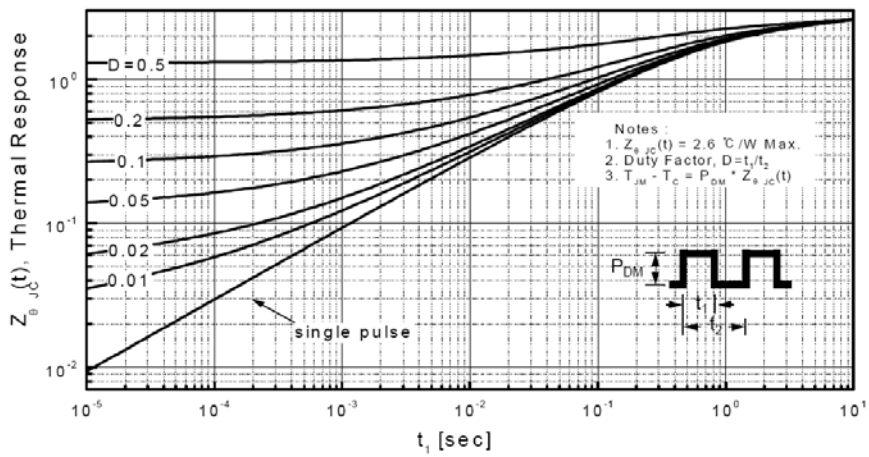
Transient Thermal Response Curve For JCS8N65FB
