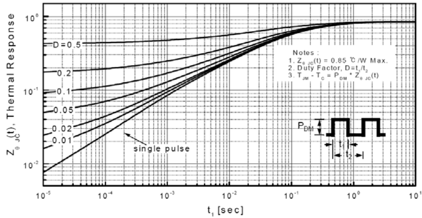
Transient Thermal Response Curve For JCS8N65FB
