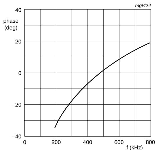
Fig 5. Typical phase of drain ringing at switch-on (at N \times V_o = 80 V)
