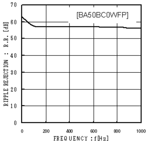
Fig.9 Ripple Rejection
