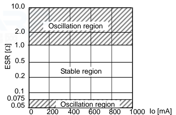
Fig.22 ESR vs. I_o (22 \mu F)
