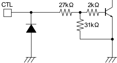
Fig.20 Input Equivalent Circuit
