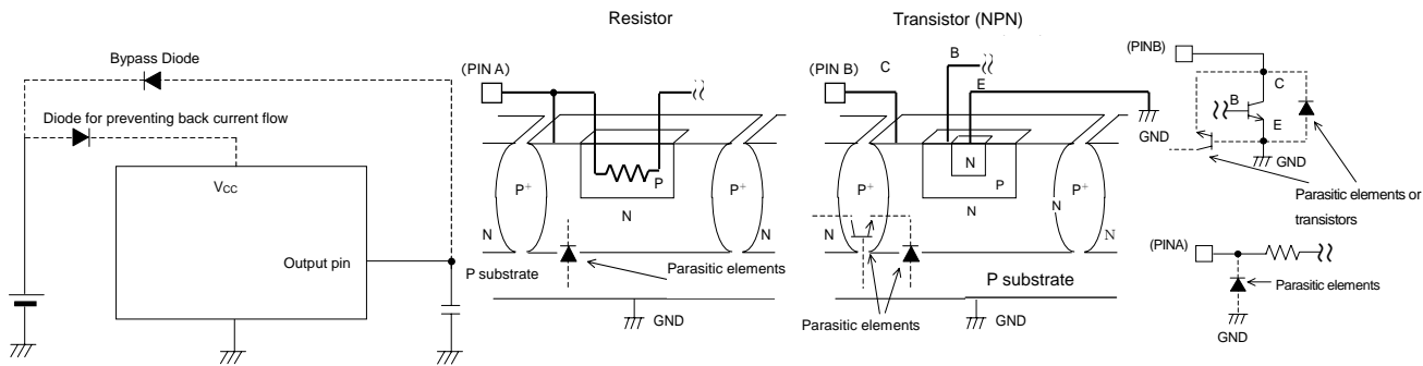
Fig.23 Bypass Diode
