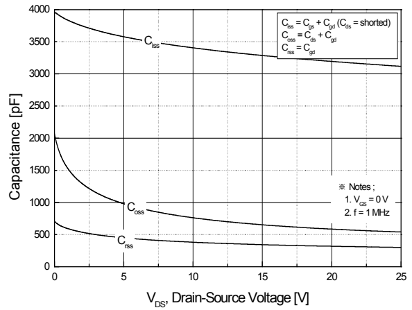
Fig.8 Capacitance Characteristics
