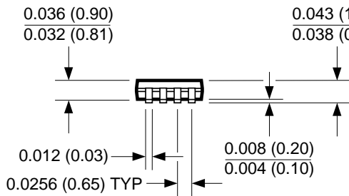
8-Lead MSOP (MM)
