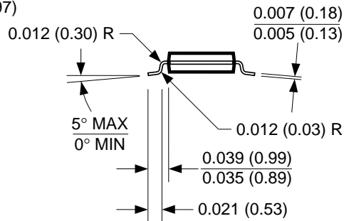
8-Lead MSOP (MM)
