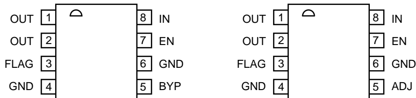
MIC5206-x.xBMM (Fixed Output Voltage)
