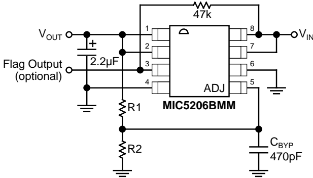
Figure 3. Ultra-Low-Noise Adjustable Voltage Application
