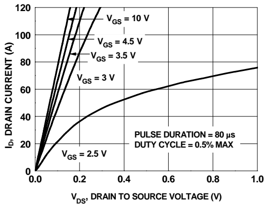
Figure 14. On-Region Characteristics
