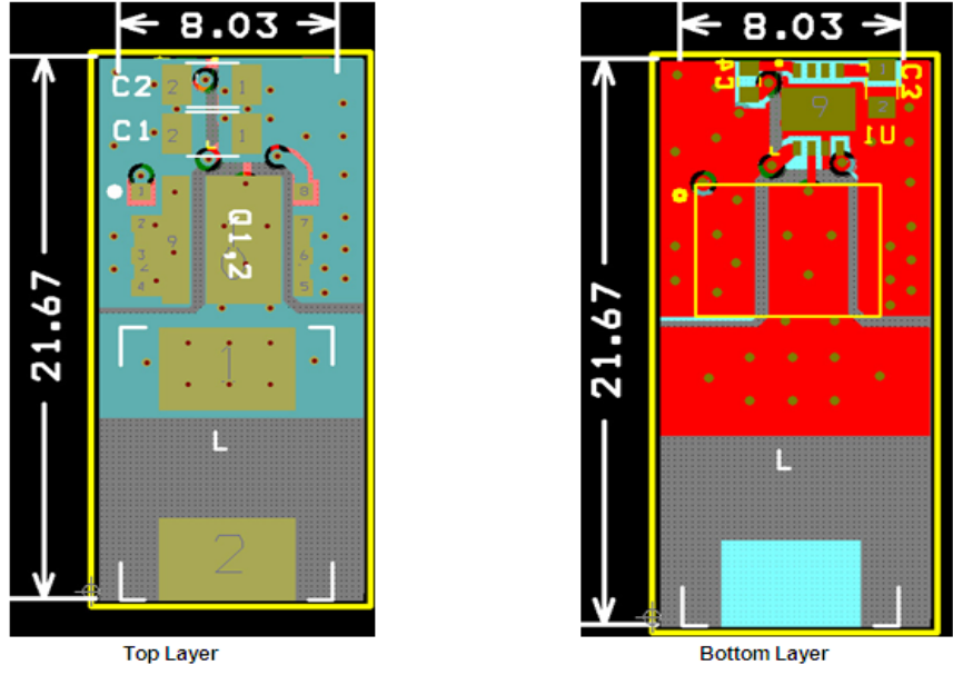
Figure 31. Recommended PCB Layout
