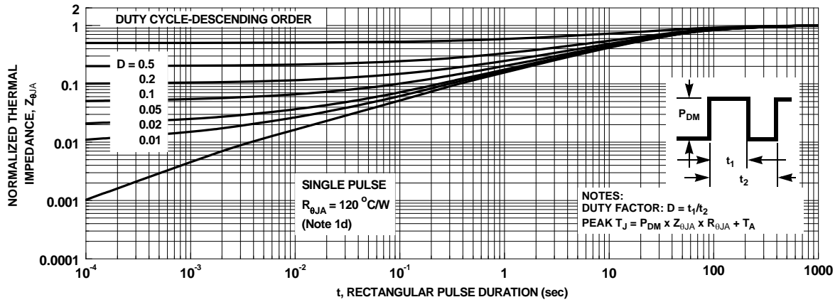
Figure 26. Junction-to-Ambient Transient Thermal Response Curve
