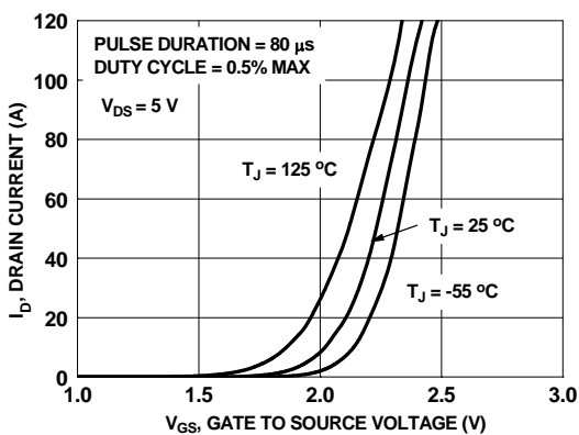
Figure 18. Transfer Characteristics
