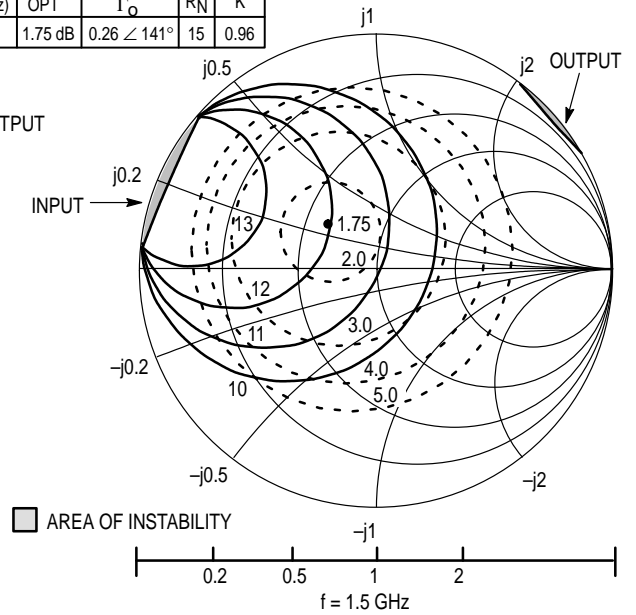
Figure 26. MRF947 Series Constant Gain and Noise Figure Contours
