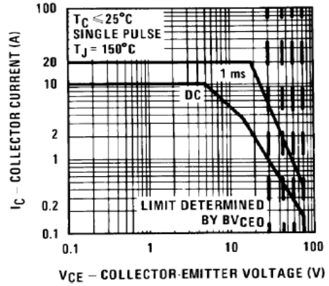
Safe Operating Area TO-220
