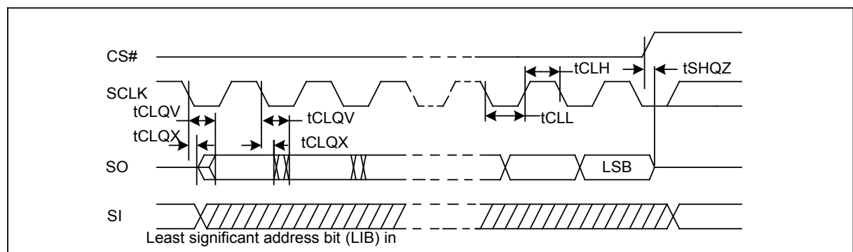
Figure 43. Output Timing
