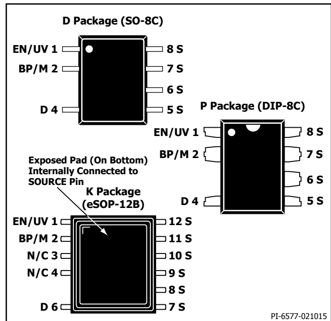
Figure 4. Pin Configuration.
