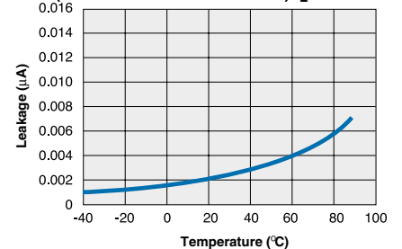
CPC1231N Typical Leakage vs. Temperature (Measured across Pins 3 & 4) I_L = \text{max rated}
