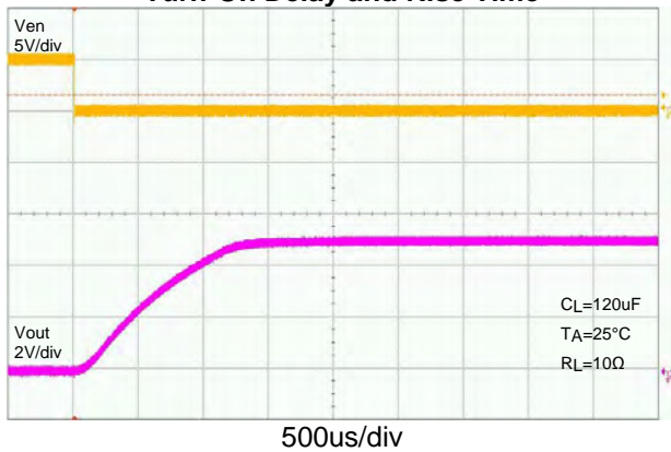
Turn-On Delay and Rise Time
