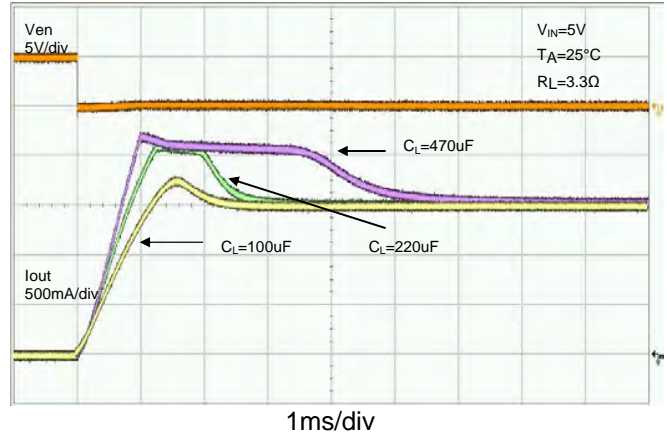
Inrush Current
